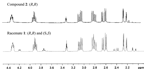
Figure 2. 1 H-NMR spectra of 1 and 2 in MeOD.
